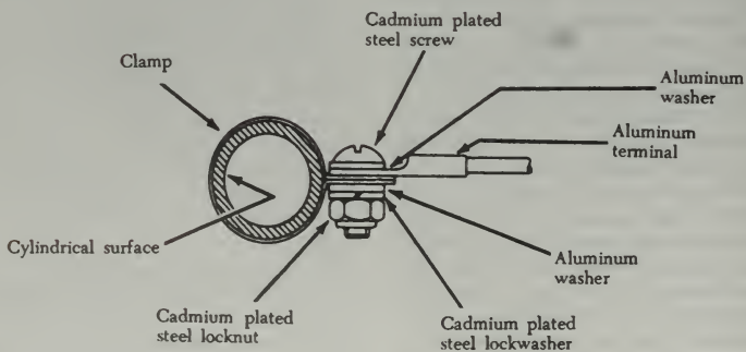
C. Aluminum jumper connection to tubular structure.
